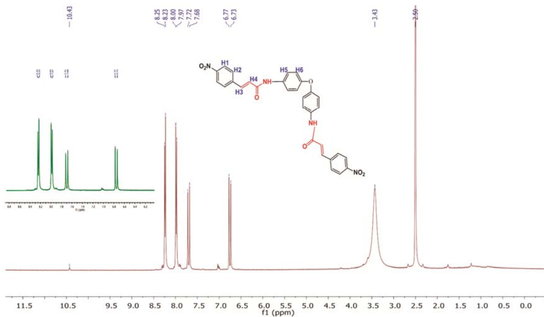
Fig S6 — 1 H NMR spectrum of compound 2
