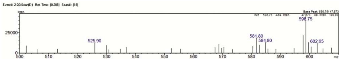
Fig S9: LS-MS/MS spectrum of compound 3
