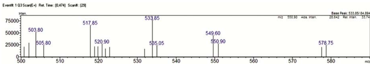
Fig S8 — LS-MS/MS spectrum of compound 2
