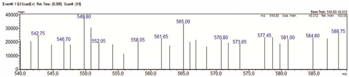
Fig S4 — LS-MS/MS spectrum of compound 1
