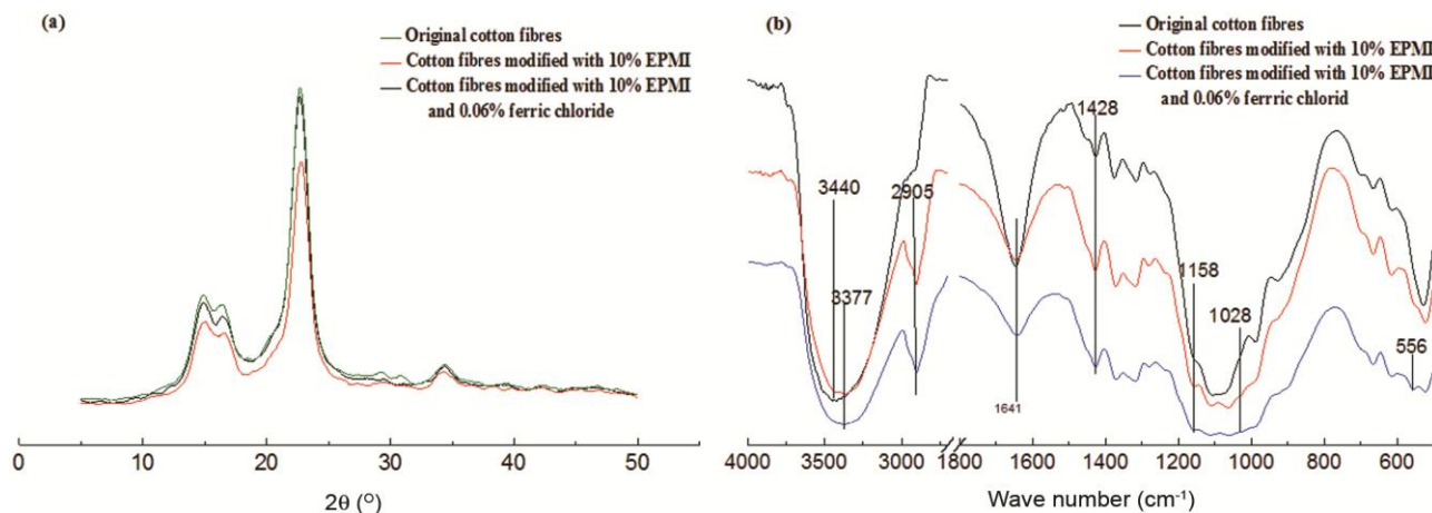
Fig. 3 — (a) XRD patterns, and (b) FTIR spectra of cotton fibers before and after modification
