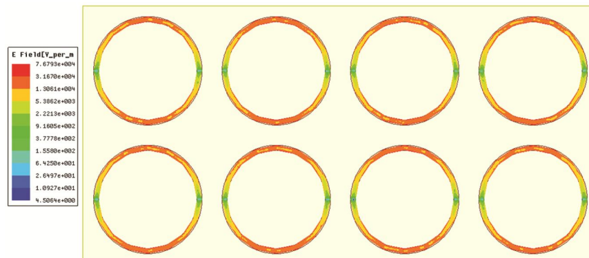
Fig. 8 – Induced electric field distributions at 2.48 GHz.
